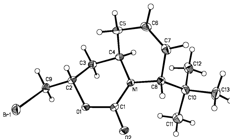
Figure 1. Molecular structure of 2b . The non-hydrogen atoms are shown with the thermal ellipsoids drawn at the 50% probability level. Hydrogen atoms have been drawn as circles of arbitrarily small radius for clarity.
